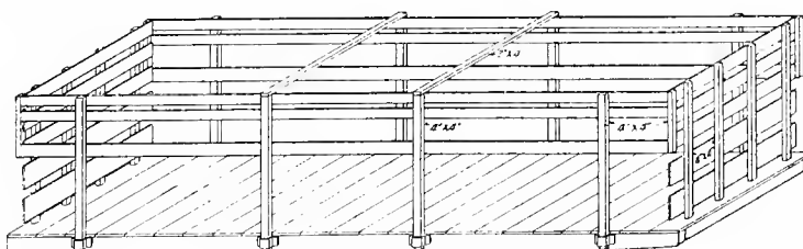
Fig. 5572. RECOMMENDED PRACTICE IN RACKING A CAR FOR LOADING BARK.
